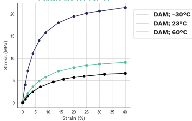
Stress-strain Pebax® MV 1074 SP 01
