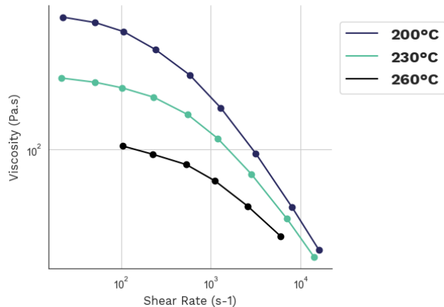
Viscosity-shear rate Pebax® MV 1074 SP 01
